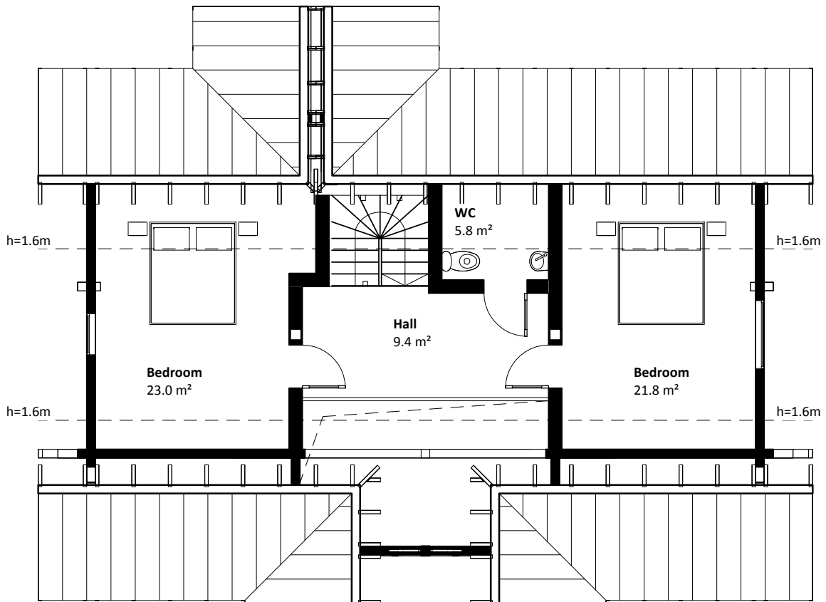
1st floor plan m 1/100
